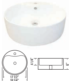
KASU - DR GBC1818 Metro White Glazed Fireclay Ceramic Top Rest with Overflow Min. Cabinet Width: 20" Strainer Not Included
